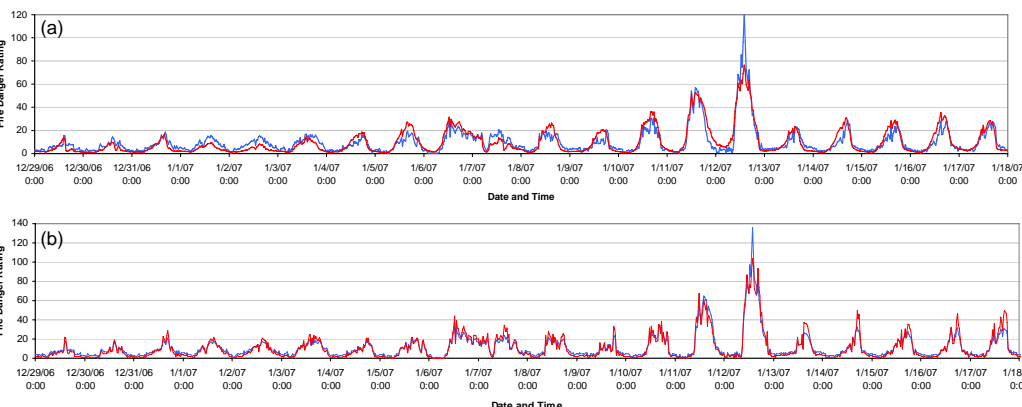
Figure 2. Time series of F^* (blue) and model predictions of fire danger rating (red). (a) McArthur's Forest Fire Danger Rating, (b) McArthur's Grassland Fire Danger Rating.
